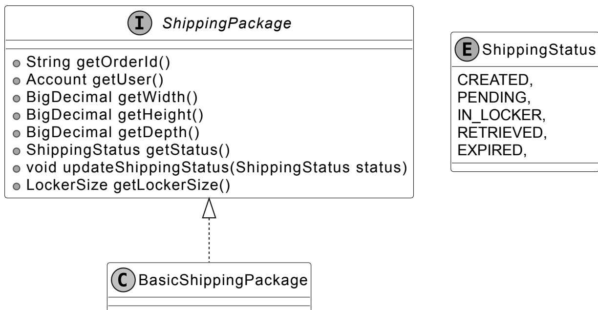
ShippingPackage interface and ShippingStatus enum
